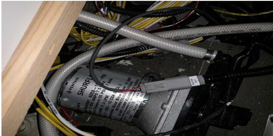
Figure 40: Fully seated heater box connector
