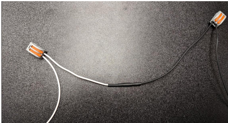
Figure 13: Diode Assembly Connected to Coach Heater Line
